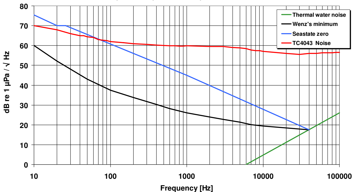
Hydrophone type TC4043 Equivalent spectral noise pressure level.
