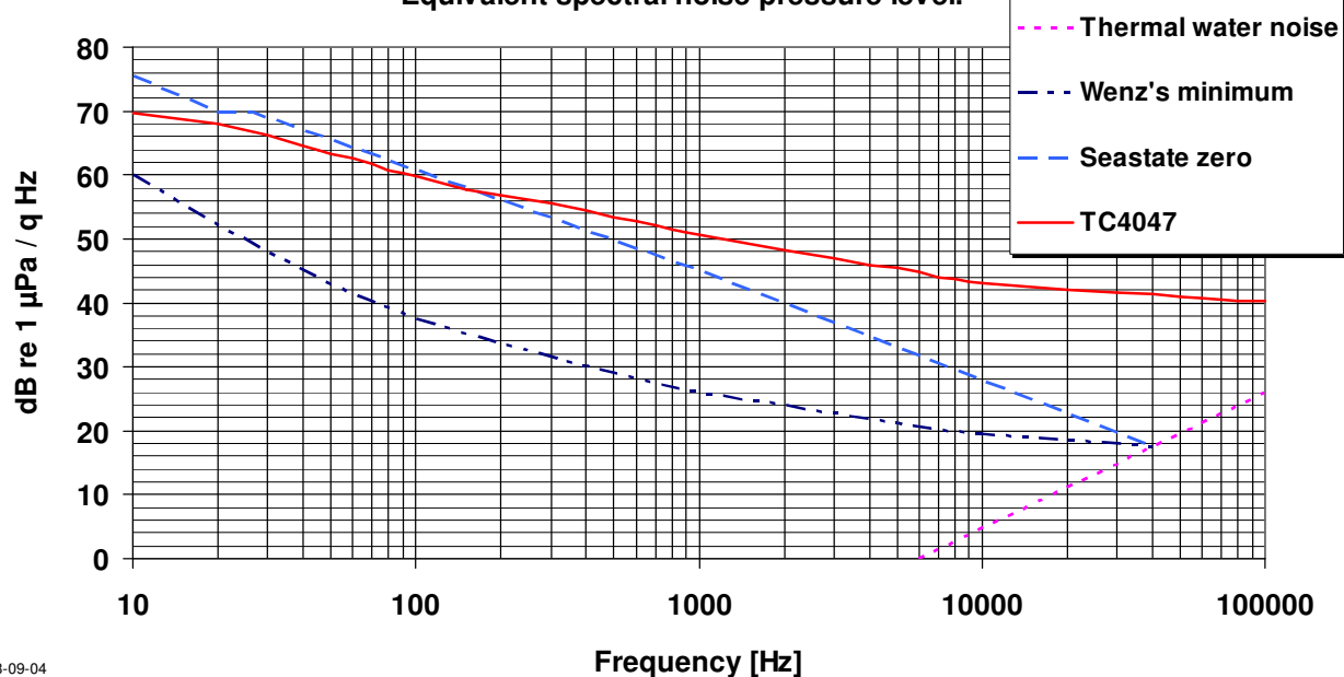
Hydrophone type TC4047 Equivalent spectral noise pressure level.
