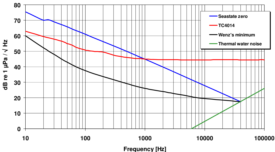
TC4014 Equivalent noise spectrum
