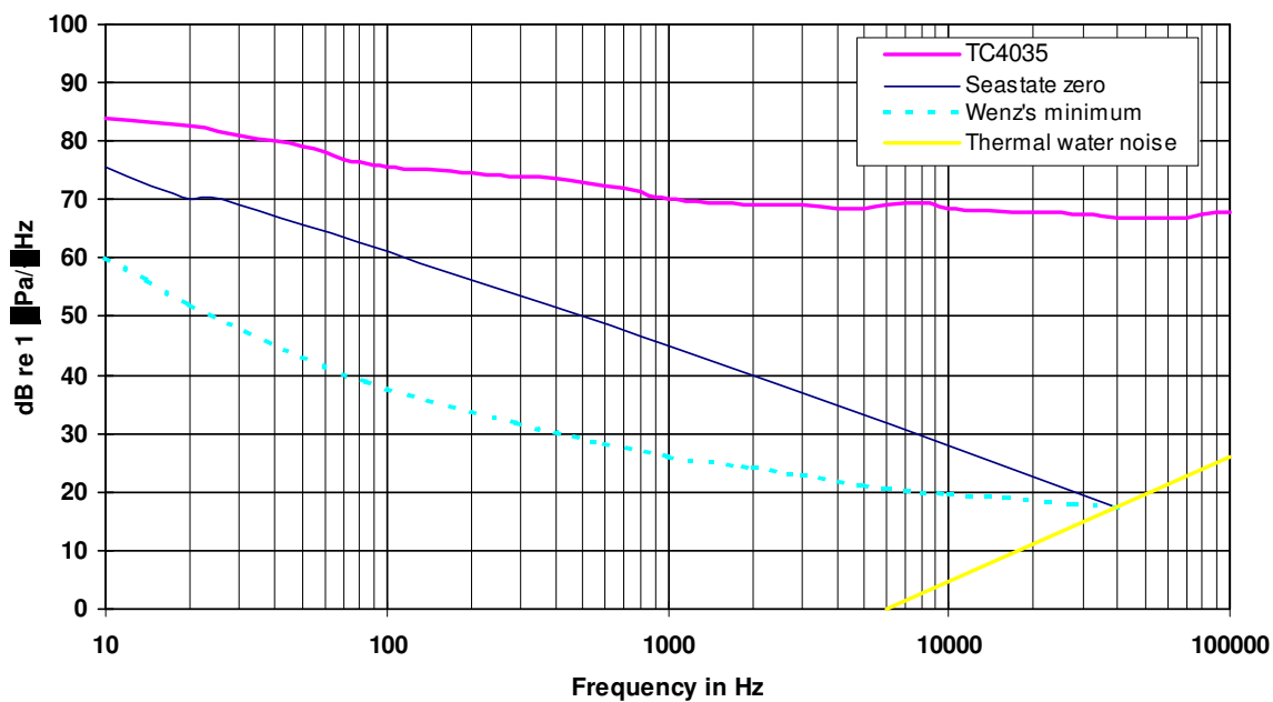
Hydrophone type TC4035 Typical equivalent noise pressure curve
